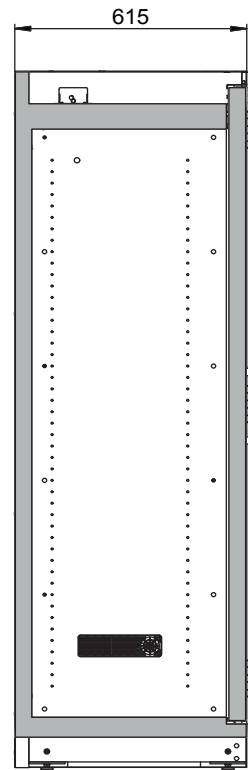
Side view
